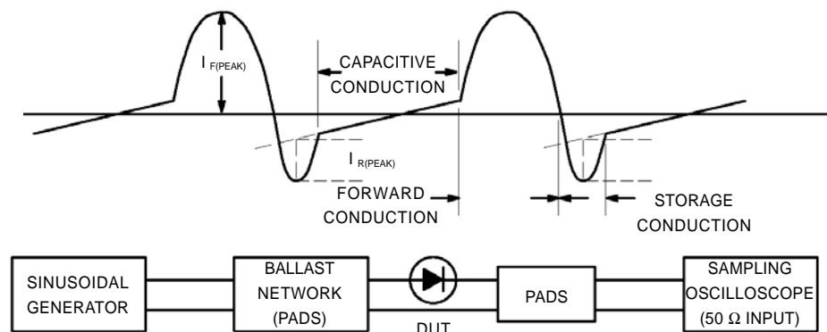
Figure 5. Krakauer Method of Measuring Lifetime
